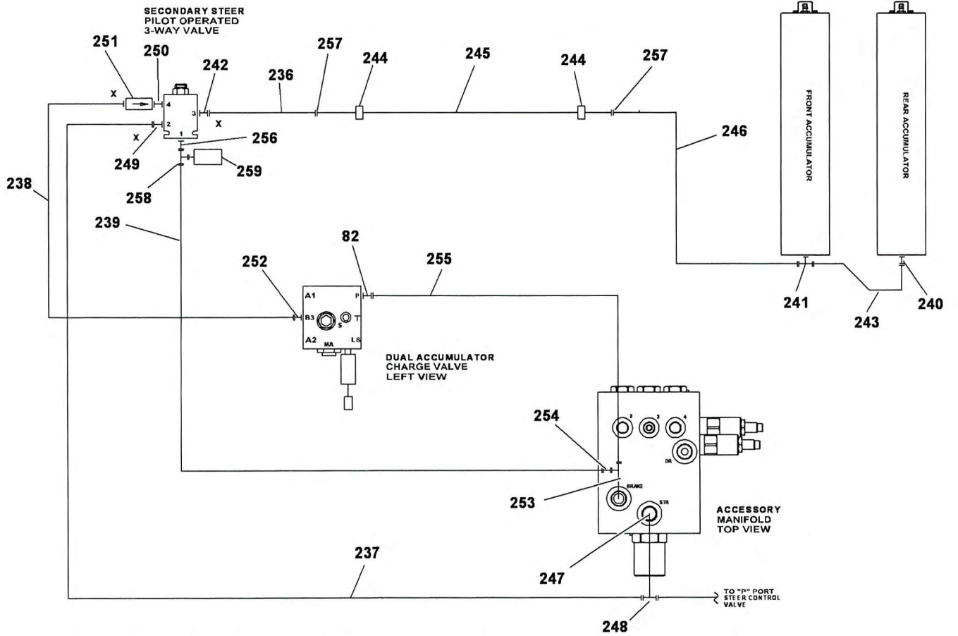
EMERGENCY FRONT STEER HYD LINES C.E.
